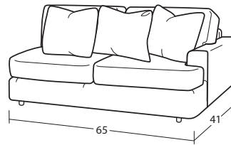
31BD RAF LOVESEAT 65W x 41D x 36H 2- 21" A Pillows 1- 21" B Pillow
